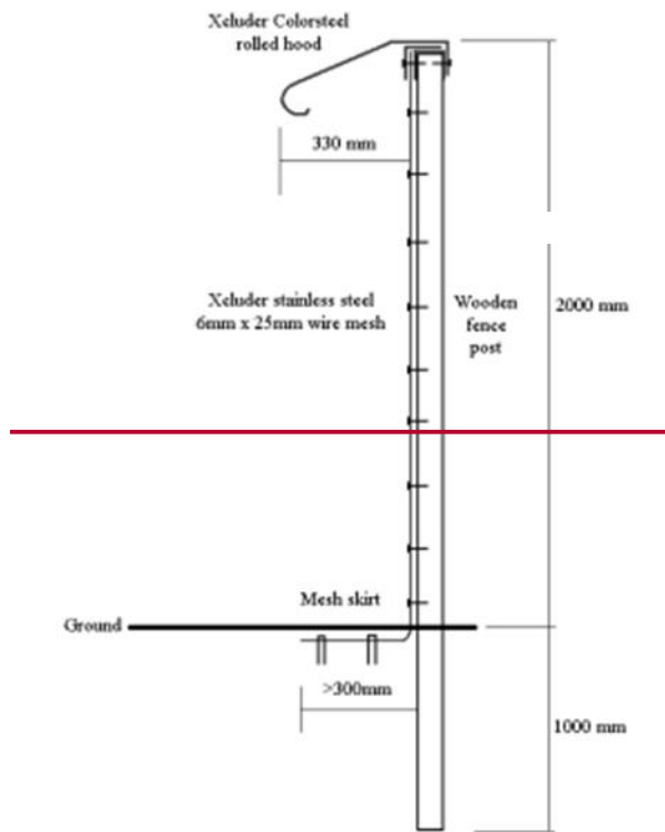
Figure 7.1 Mouse, rat, mustelid, possum and cat proof fence design
